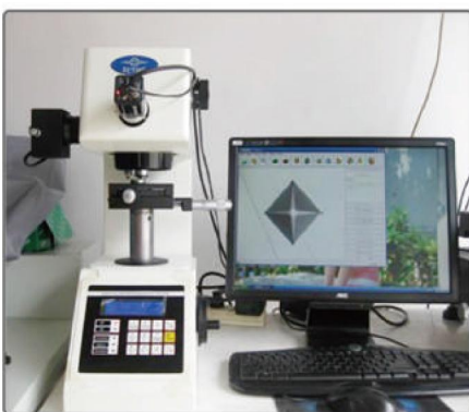
维氏硬度计 Digital micro vickers hardness tester
